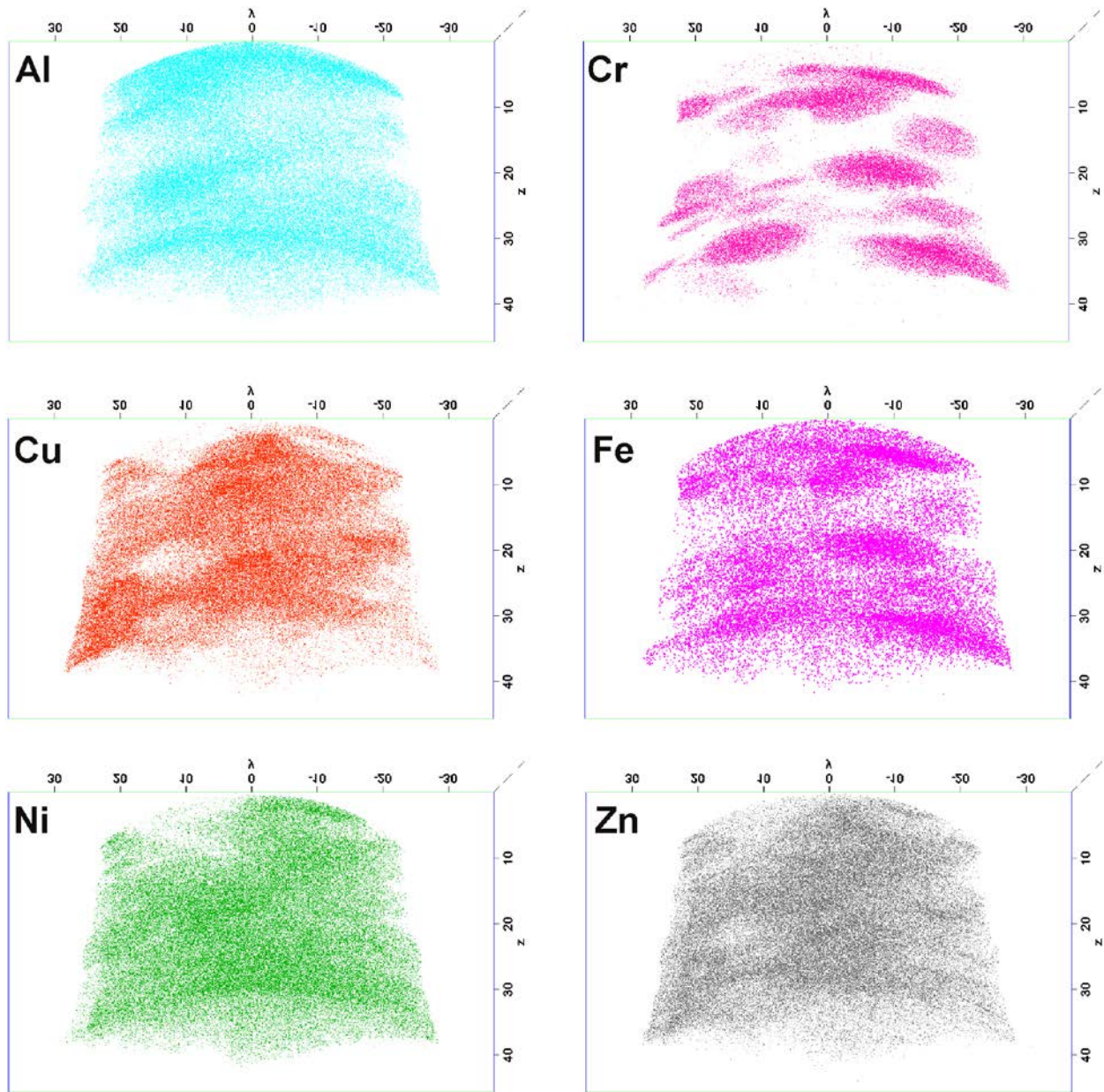
Fig. 7. APT elemental map displaying the atomic positions of Al, Cr, Cu, Fe, Ni, and Zn in an analyzed volume of 74 \times 74 \times 46 \text{ nm}^3 of hot compacted AlCrCuFeNiZn HEA (600 °C for 15 min at 650 MPa).
