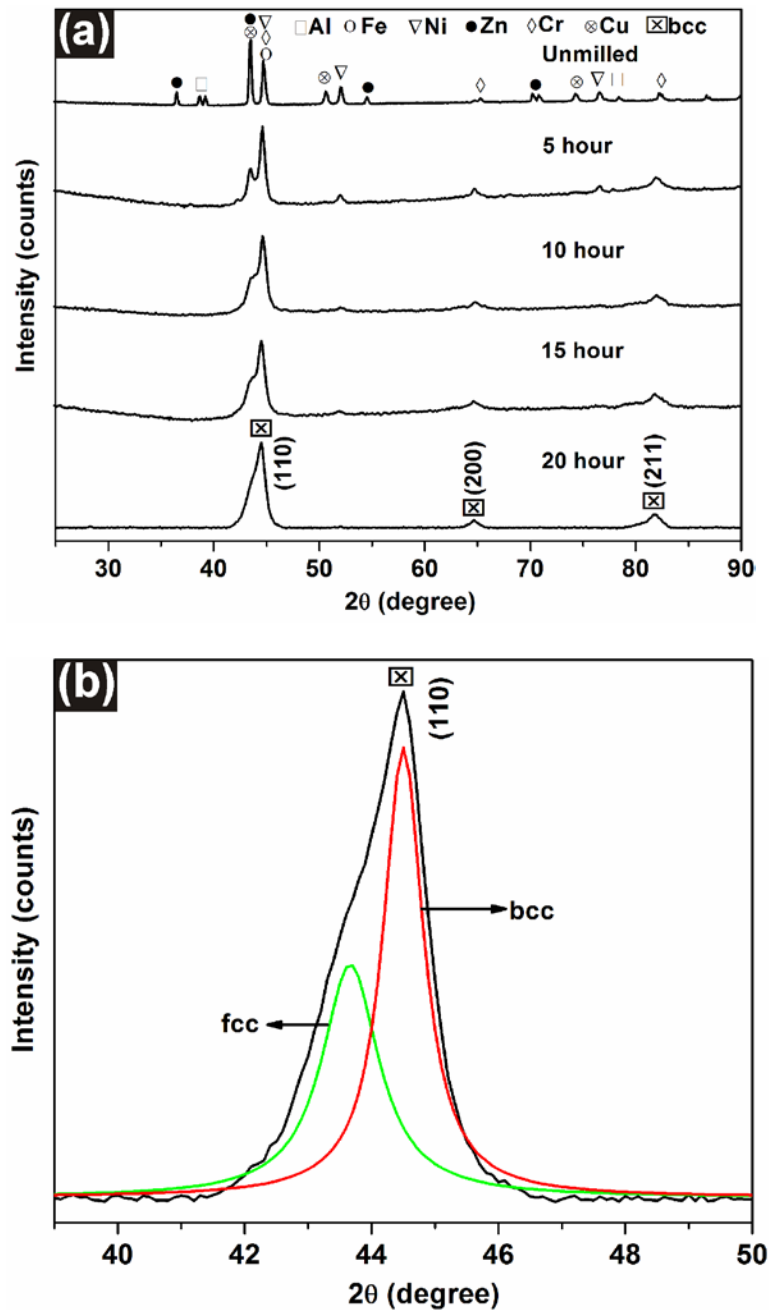
Fig. 1. X-ray diffraction pattern of the AlCrCuFeNiZn HEA powder samples (a) obtained after accumulative milling intervals of 5 h ( \text{Cu } K_{\alpha 1} , \lambda = 154 pm); (b) deconvoluted high intensity (110) peak corresponding to the major bcc phase ( a_{\text{bcc}} = 267 pm) obtained after 20 h milling, also showing the presence of a minor fcc phase peak corresponding to the (111) plane with lattice parameter a_{\text{fcc}} = 367 pm.
