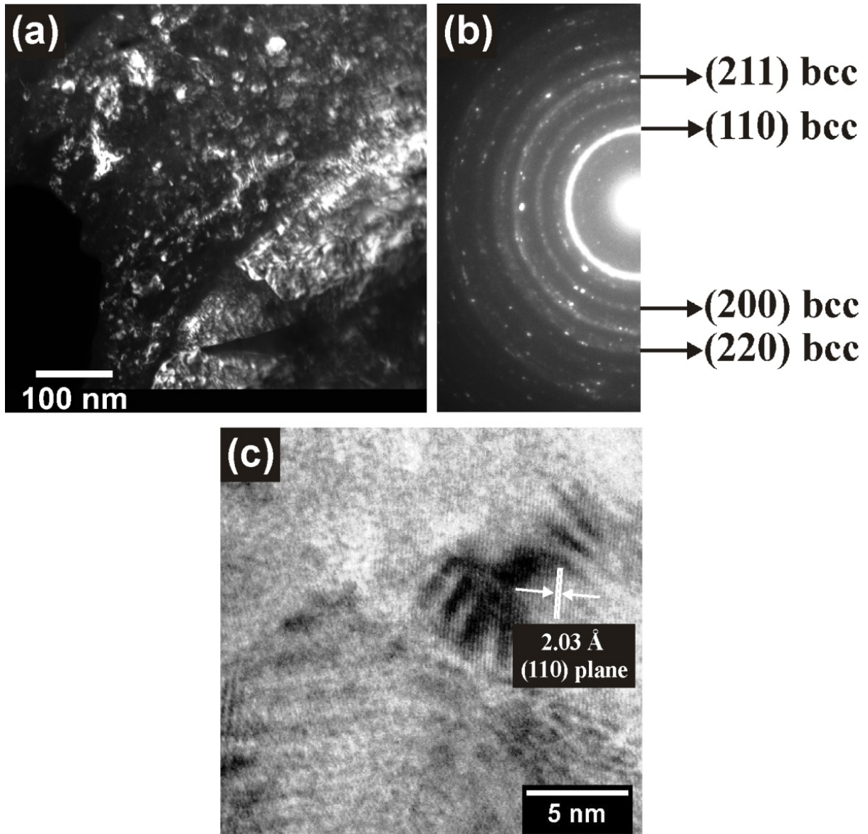
Fig. 2. (a) DF TEM image of the 20 h milled AlCrCuFeNiZn HEA powder using the (110) diffraction ring; (b) corresponding SAED pattern showing the diffraction rings of the bcc phase; (c) HRTEM image of a region with atomic planes corresponding to the bcc phase with an interplanar spacing of 203 pm.
