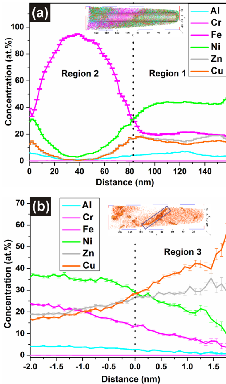
Fig. 6(a). Concentration-depth profiles of all alloying elements in the hot compacted (600 °C for 15 min at 650 MPa) AlCrCuFeNiZn HEA taken along the analyzed volume of 46 \times 46 \times 180 \text{ nm}^3 (inset). Concentration values are determined in 2 nm thick slices with a radius of 12 nm. The profiles are plotted with a moving step of 2 nm from right to left. The dotted lines separate regions 1 and 2 which are enriched in Ni and Fe, respectively. (b) Proximity histogram of 0.1 nm bin size with respect to the selected Cu-Zn phase boundary (with 28 at. % Cu interface) marked with a rectangle in the inset.
