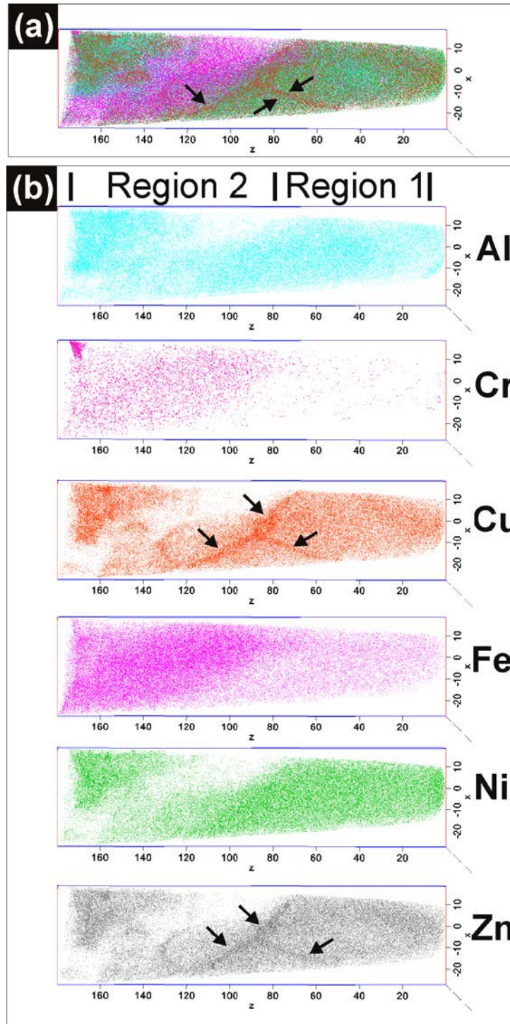
Fig. 5. APT data of hot compacted (600 °C 650 MPa for 15 min) AlCrCuFeNiZn HEA: (a) Elemental map displaying the overall distribution of atoms; (b) three-dimensional reconstruction of individual Al, Cr, Cu, Fe, Ni, Zn atom positions in an analyzed volume of 46 \times 46 \times 180 \text{ nm}^3 . The arrows indicate the segregation of Cu and Zn atoms along the grain boundaries.
