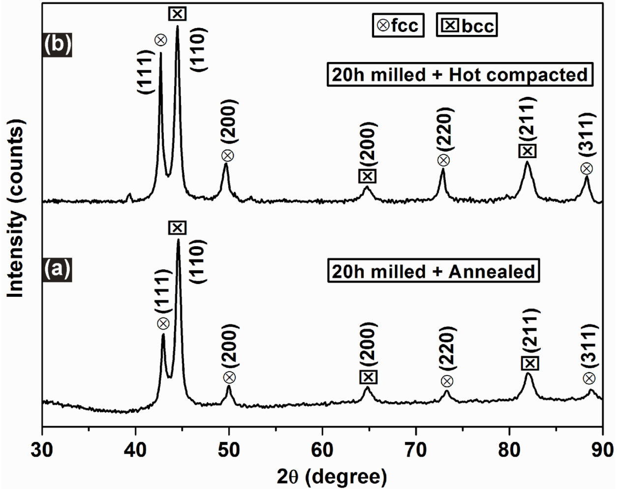
Fig. 3. X-ray diffraction pattern (Cu K_{\alpha 1} , \lambda = 154 pm) of the 20 h milled AlCrCuFeNiZn HEA powder after: (a) annealing at 600 °C for 15 min; (b) hot compaction at 600 °C with 650 MPa for 15 min.
