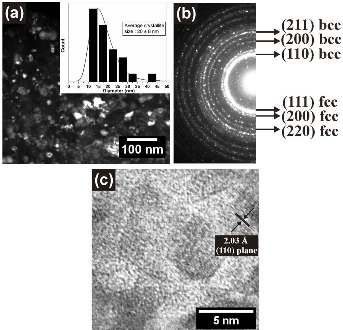
Fig. 4. TEM images of hot compacted (600 °C for 15 min at 650 MPa) AlCrCuFeNiZn HEA: (a) Dark field micrograph imaged using the (110) diffraction ring showing fine nanocrystals. Inset showing histogram of crystallite size. Continuous curve displays fit using log-normal distribution function; (b) corresponding SAED pattern showing the diffraction rings corresponding to the bcc and fcc phases; (c) HRTEM image of a region showing atomic planes corresponding to the bcc phase with an inter-planar spacing of 203 pm.
