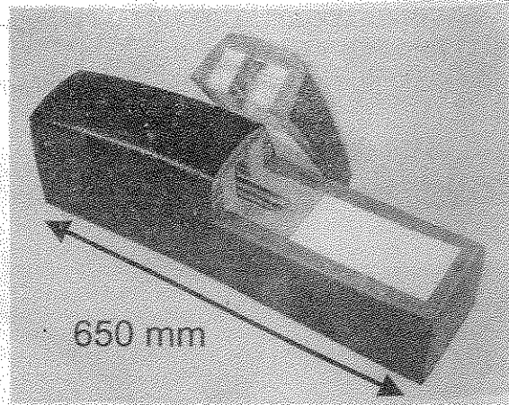
Fig. 2(a) : Prototypes of crash absorbers based on Al extrusions with a filling of Cymat aluminium foam. 2(b) Crash energy absorber for a tram built for the COMBINO vehicle system.
