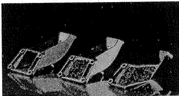
Fig. 3: Prototype of a BMW engine mounting bracket manufactured by LKW Ranshofen. From left; empty casting, composite part consisting of foam core and cast shell, section through composite part.
