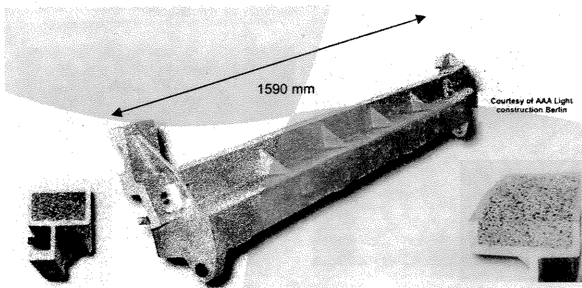
Fig. 4: Transverse beam of a machine. Two insets show cross sections in different direction of the beam.
