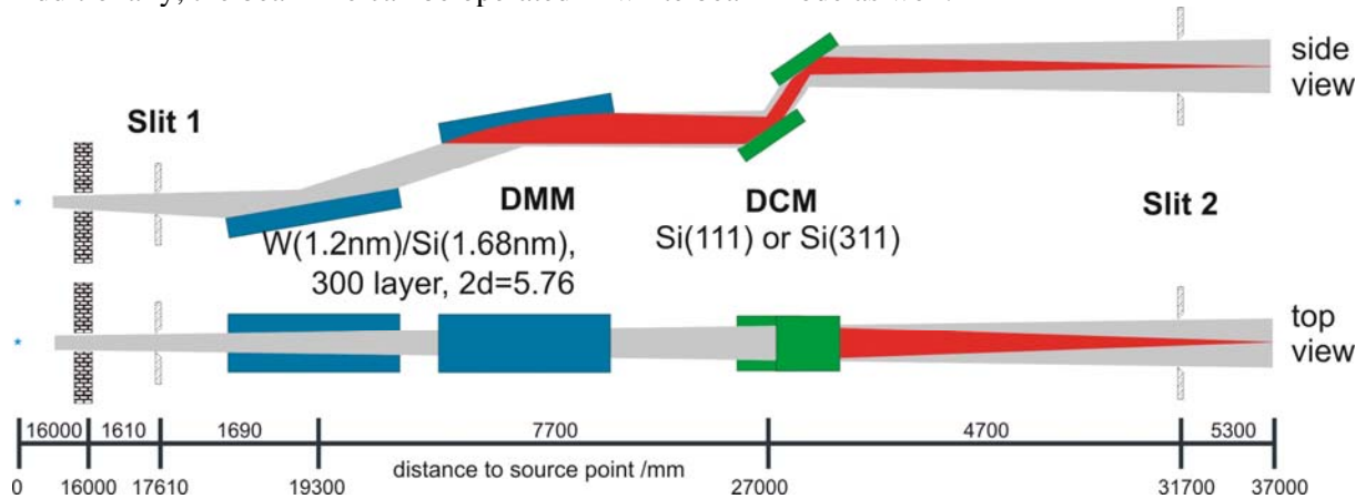
Figure 1. Principle sketch of the BAMline's X-ray beampath (top: side view, bottom: top view). The radiation originating from the insertion device (7T-WLS) can be monochromatized using a double multilayer monochromator (DMM) and/or a double crystal monochromator (DCM) which includes a vertical focusing option for the DMM and a horizontal for the DCM. The position of the tomography stage is in the experimental hutch at a distance of 35 m from the source [1, 2].
