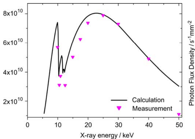
Figure 2. Photon flux density behind the double multilayer monochromator at the BAMline; measured and calculated (using Reflec) with a ring energy of 1.7 GeV, a ring current of 200 mA, a magnetic flux density of 7 T at the wavelength shifter and a distance from the source of 35 m. At 7 keV a flux density of was measured with a focused beam. Around 11 keV typical flux reduction due to the tungsten L absorption edges can be seen (the multilayer coating consists of 150 double layers W/Si) [1, 2].
