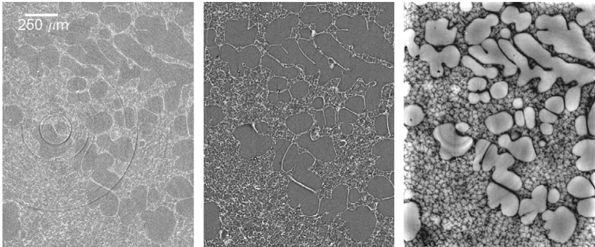
Figure 3. Left: absorption tomogram from a specimen consisting of the alloy AZ91 (magnesium and aluminium, similar attenuation coefficients), middle: same slice but as phase contrast tomography calculated from Fresnel-propagated projection images (edge enhancement), right: holotomography of this slice combining different propagation distances [3].
